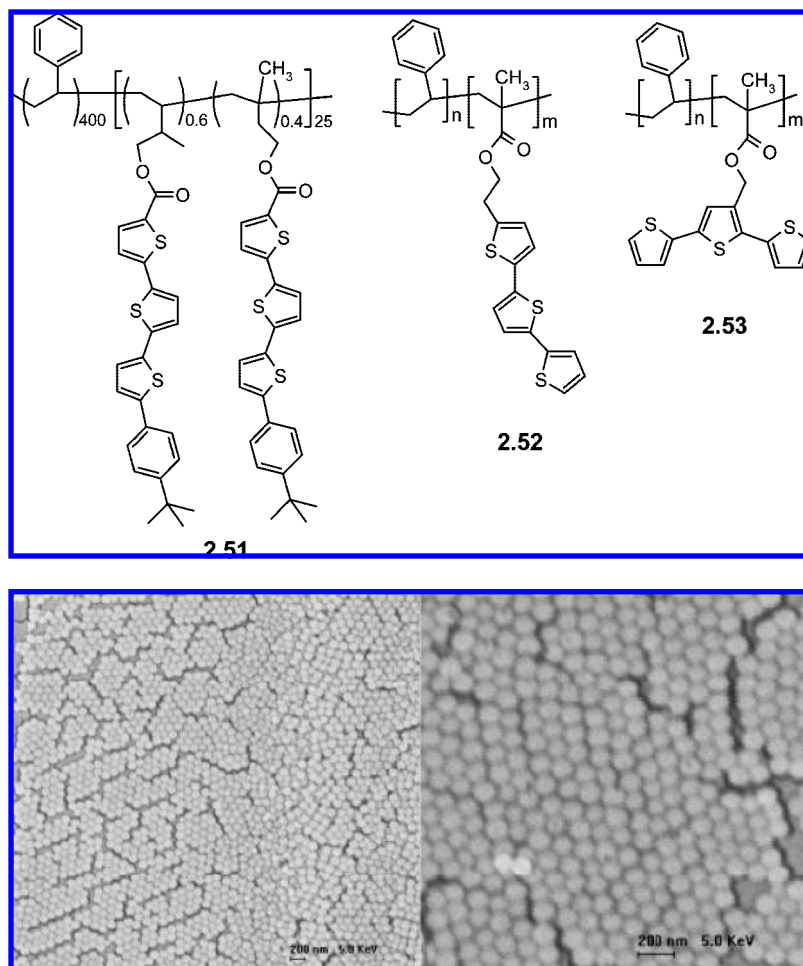
Figure 2.2. SEM micrograph images of microfluidic-induced self-assembly of nanobeads formed from copolymer 2.52 . (Reproduced with permission from ref 109. Copyright 2005 American Chemical Society.)
