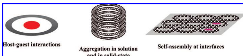
Figure 4.1. Properties of shape-persistent macrocycles.
